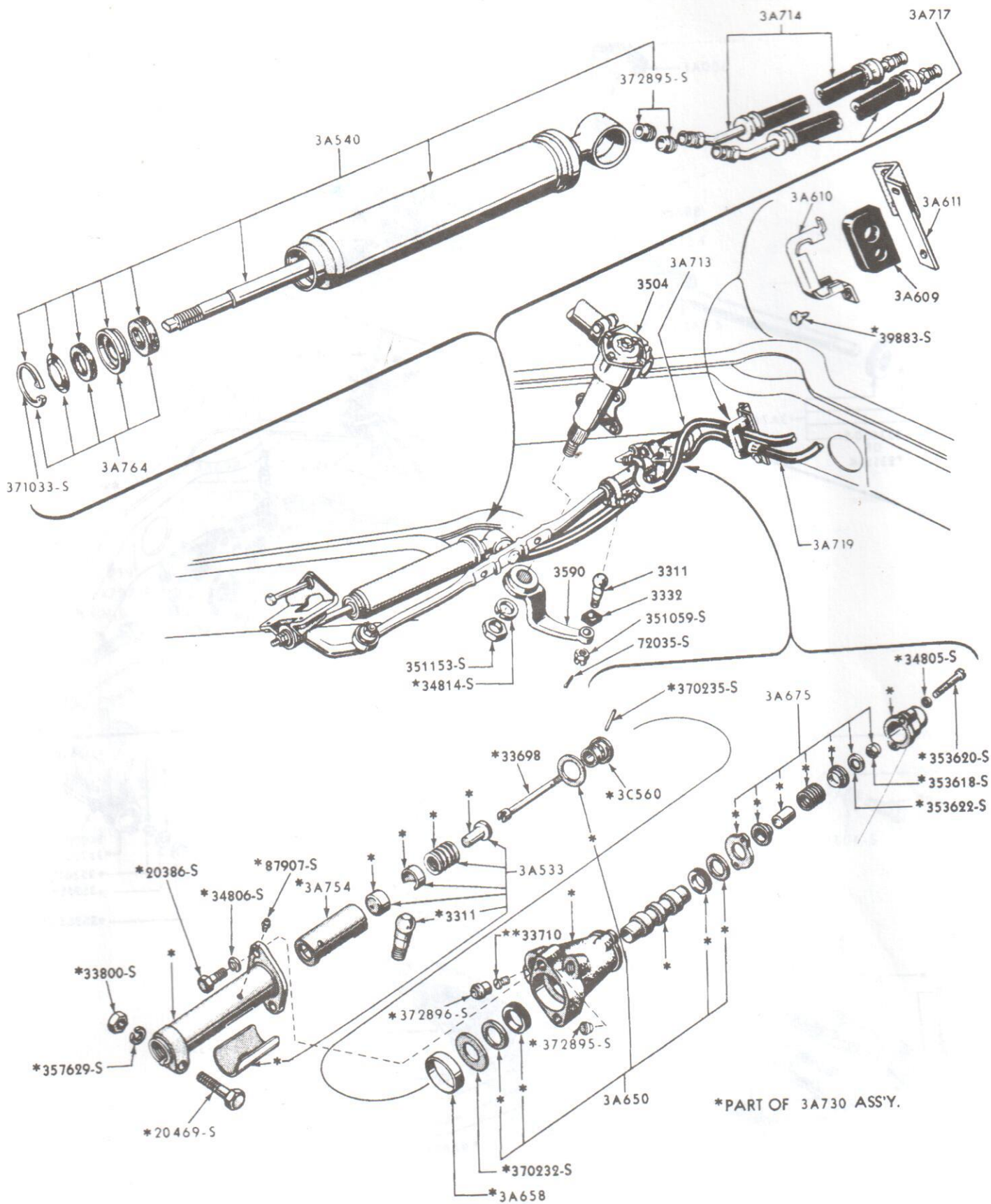
1957 Thunderbird Power Steering Valve & Cylinder
