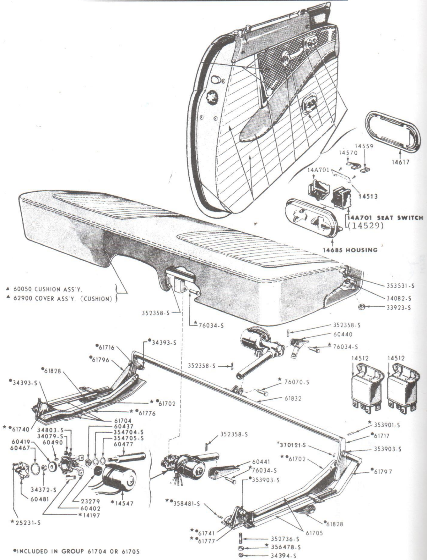
1955/57 Thunderbird Seat Assembly With 4-Way Power Regulator
