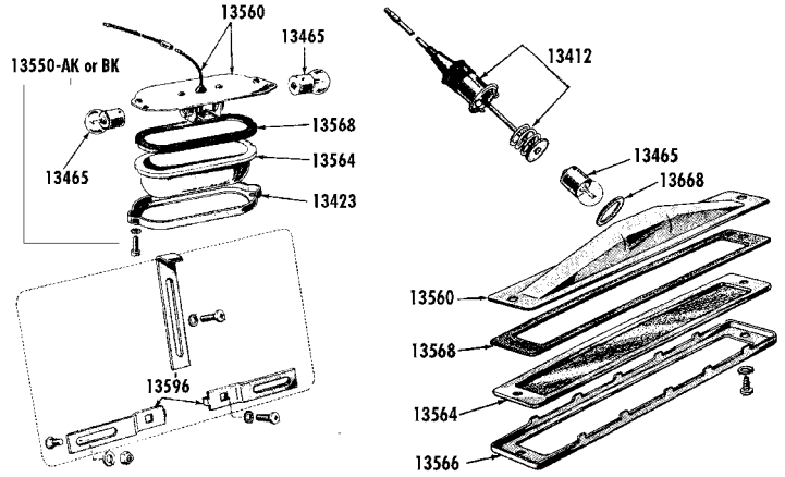
'55/56 License Lamp & Plate Holder
