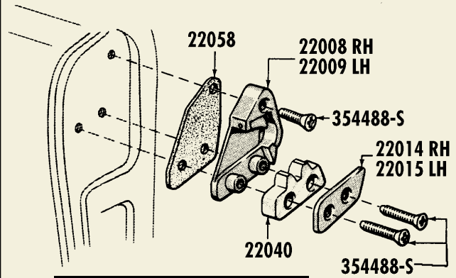
'56/57 Striker Plate Assembly
