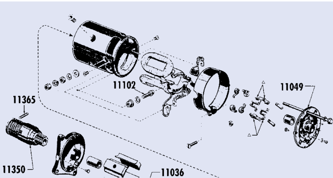
Typical (12v)
