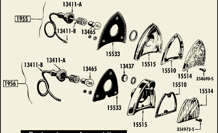
Backup Lamp Assemblies
