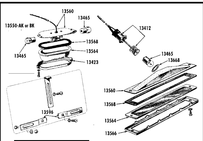
'57 Tail Lamp Assembly
