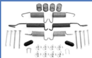
B 2095BK Brake Spring Kit
